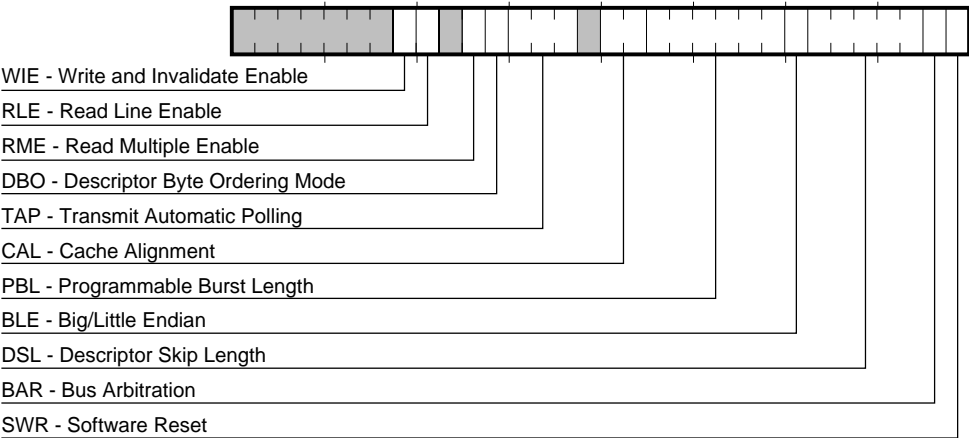
Figure 3–11 CSR0 Bus Mode Register
