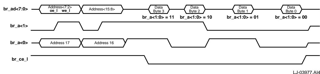
Figure 7–4 Boot ROM Dword Read Cycle
