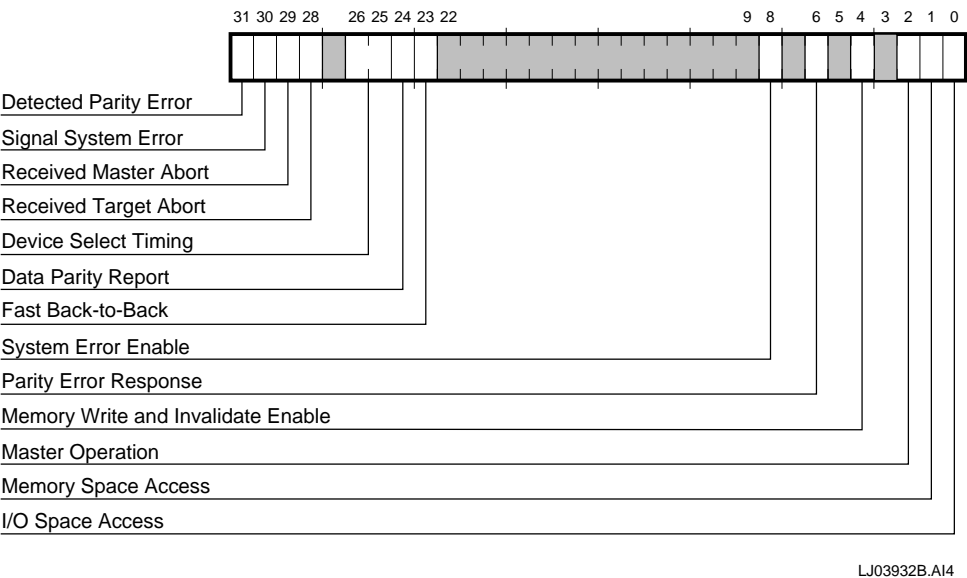
Figure 3–2 CFCS Command and Status Configuration Register
