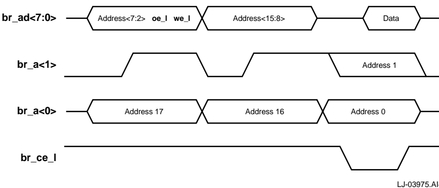
Figure 7–2 Boot ROM Byte Read Cycle
