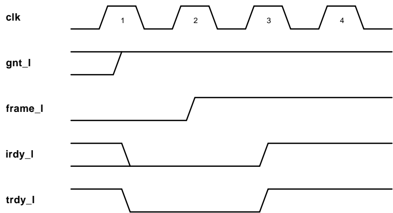
Figure 5–8 Normal Completion
