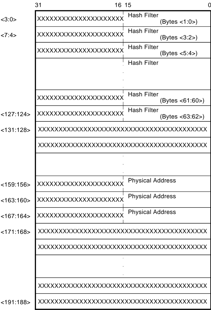
Figure 4–14 Imperfect Filtering Setup Frame Format
