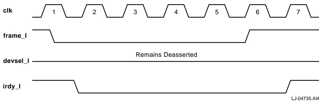
Figure 5–9 Master Abort
