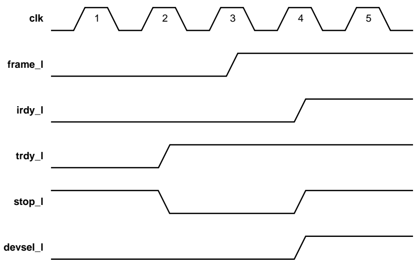
Figure 5–12 Target Retry
