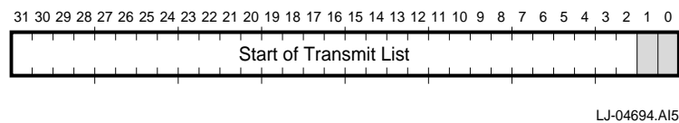
Figure 3–15 CSR4 Transmit List Base Address Register
