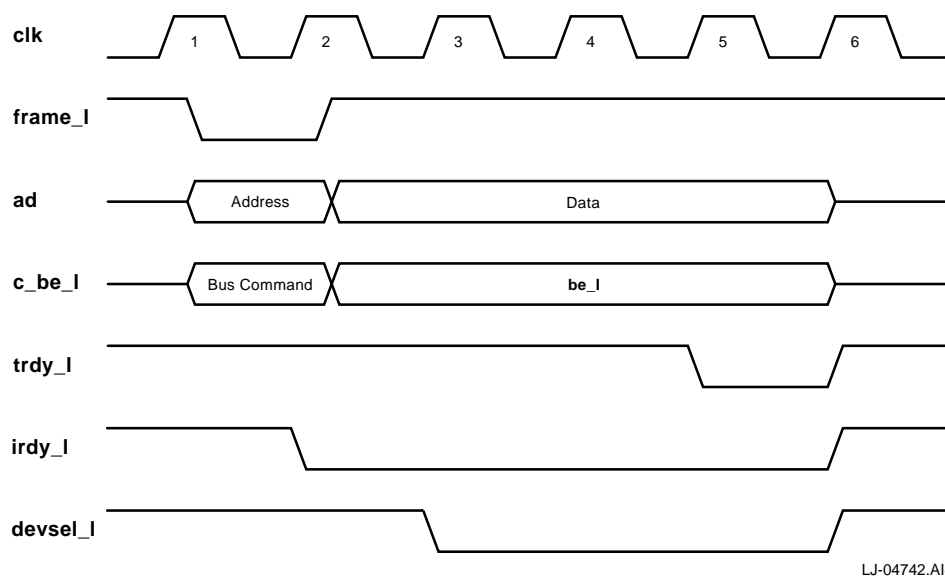
Figure 5–2 Slave Write Cycle
