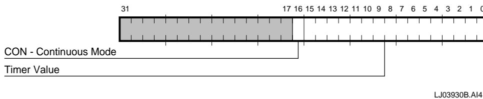
Figure 3–22 CSR11 General-Purpose Timer Register
