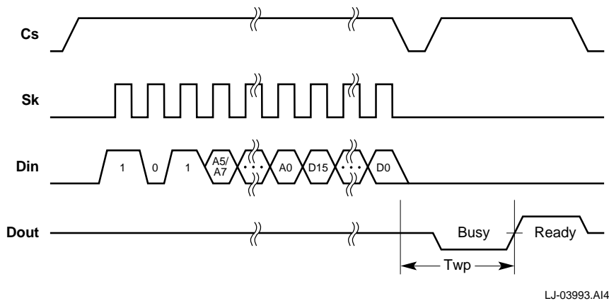
Figure 7–10 Write Operation
