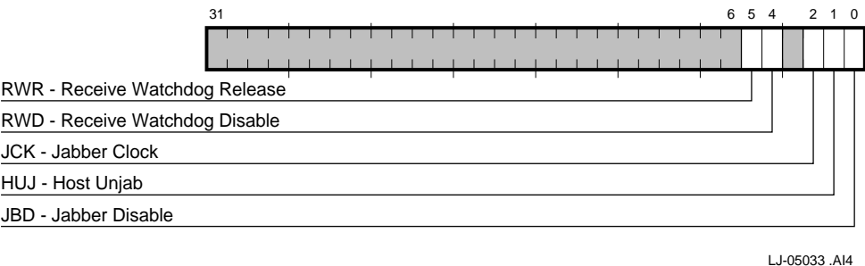
Figure 3–24 CSR15 Watchdog Timer Register
