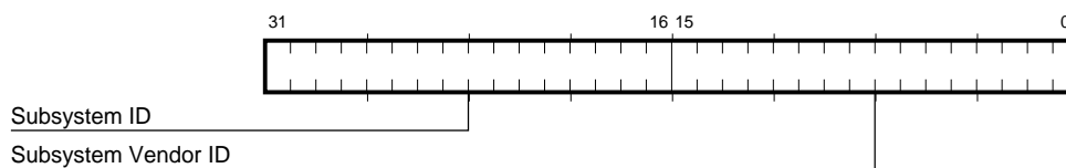
Figure 3–7 SSID Subsystem ID Register
