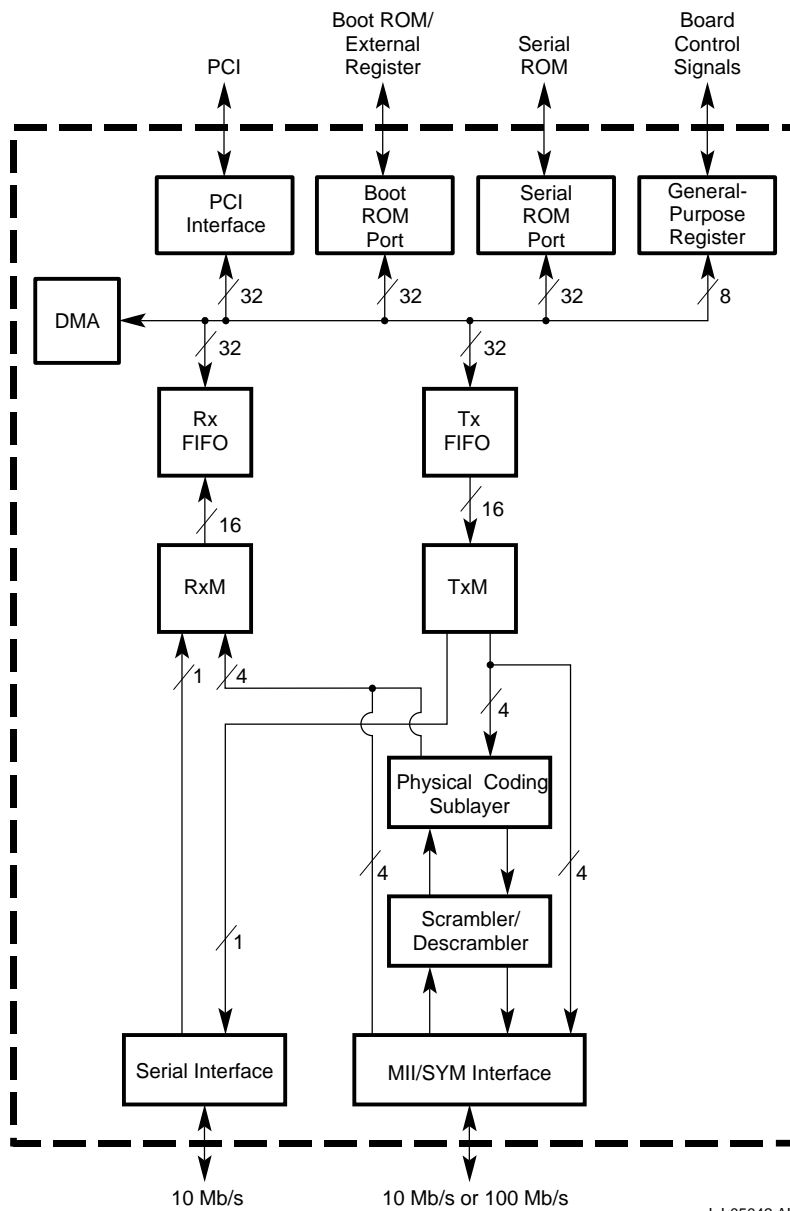
Figure 1–1 21140A Block Diagram
