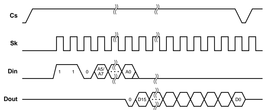
Figure 7–7 Read Operation
