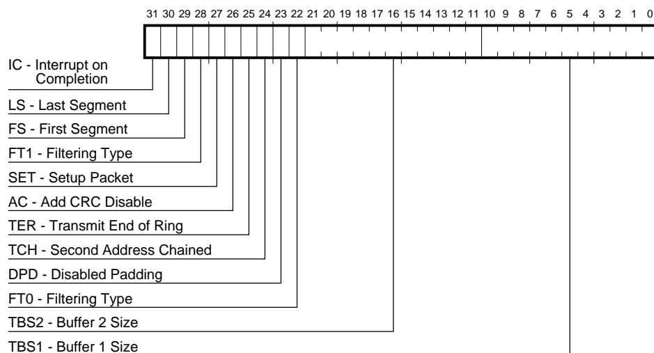
Figure 4–9 TDES1 Transmit Descriptor 1
