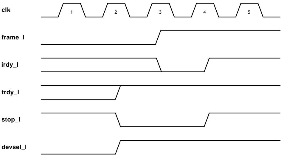
Figure 5–10 Target Abort
