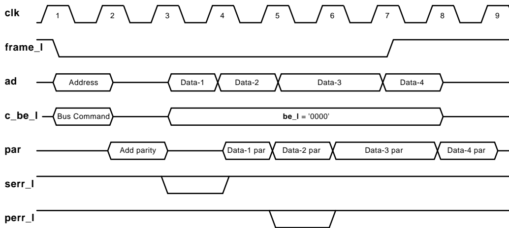
Figure 5–13 Parity Operation
