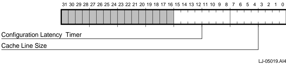
Figure 3–4 CFLT Configuration Latency Timer Register
