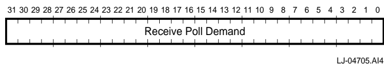
Figure 3–13 CSR2 Receive Poll Demand Register
