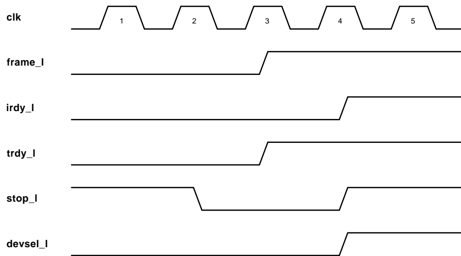
Figure 5–11 Target Disconnect
