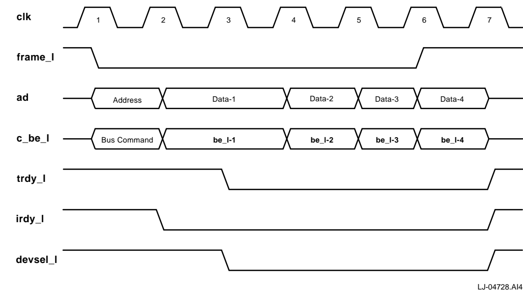
Figure 5–6 Memory Write
